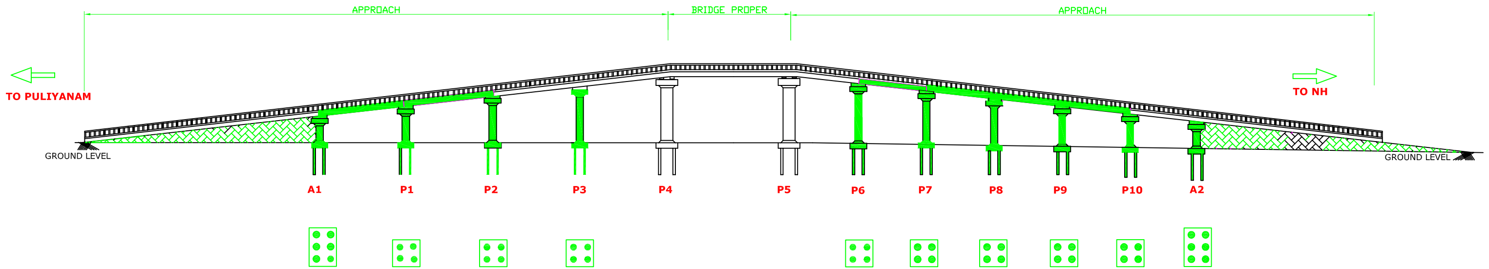
PILE FOUNDATION
